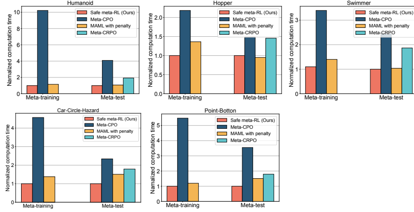
Figure 5: Normalized computation time of the meta-training and the meta-test in Humanoid, Hopper, Swimmer, Car-Circle-Hazard, and Point-Button.
