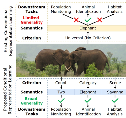
Figure 1: Existing conventional representation learning learns a universal representation that prioritizes the dominant semantics while overlooking other meaningful features, limiting their adaptability to customized tasks. In contrast, our proposed conditional representation learning (CRL) extracts representations conditioned on specific criteria, enhancing its applicability.
