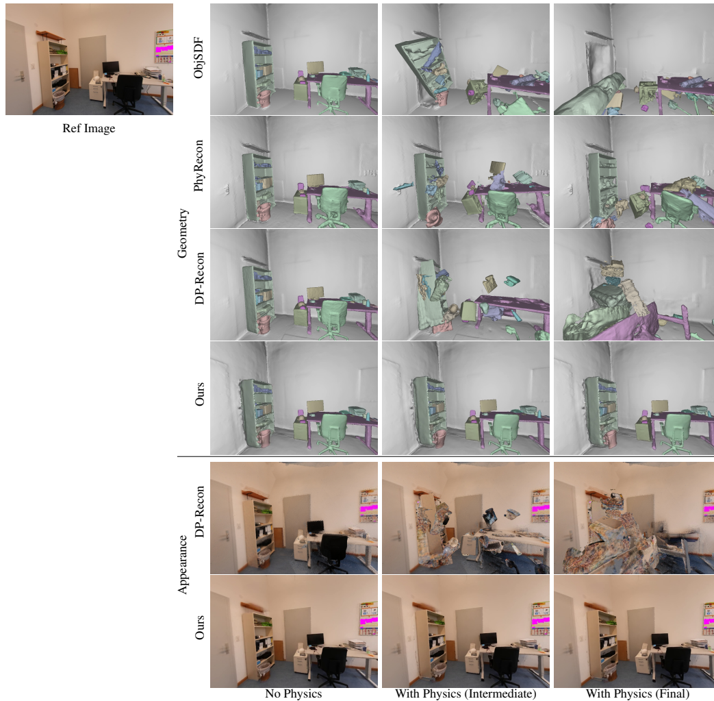
Figure 5: More Physical Simulation Results in Scannet++ Dataset Scene 1: We show the geometry and appearance of each object in the scene with physical simulation, from no physics state, intermediate state with physics, and final state with physics.
