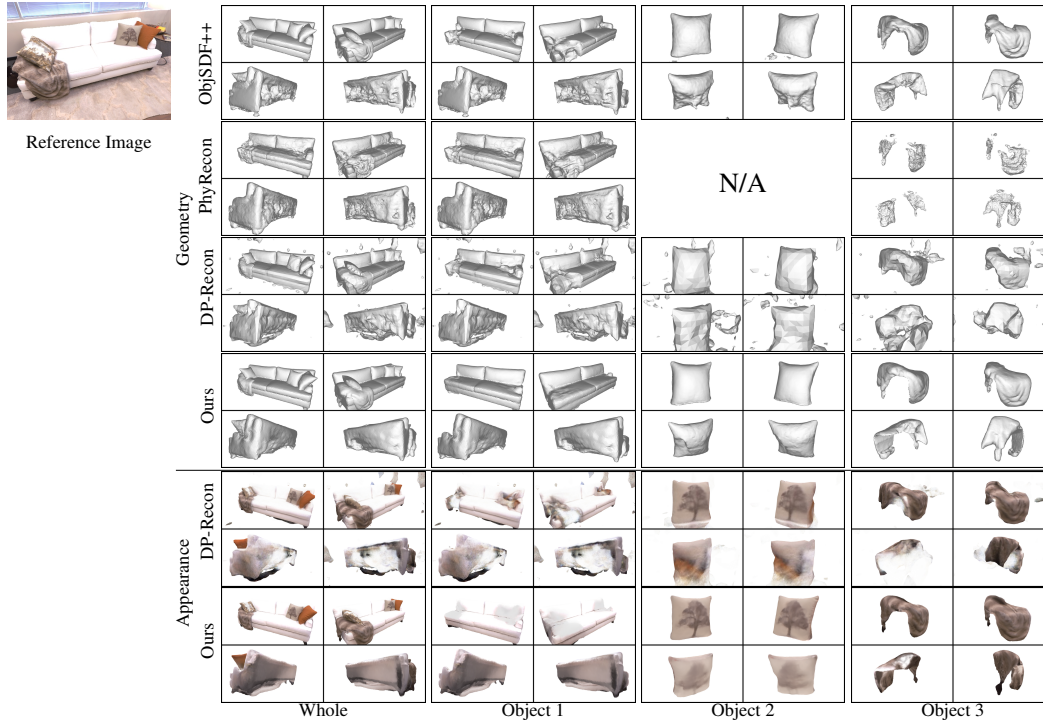
Figure 3: Qualitative Comparisons on Object Geometry and Appearance Reconstruction: Our method delivers superior reconstructions by smoothly inpainting occluded regions with LaMa and completing invisible back-facing geometry with Wonder3D. Unlike baselines, our approach eliminates object interpenetration, ensuring physical stability during simulation.
