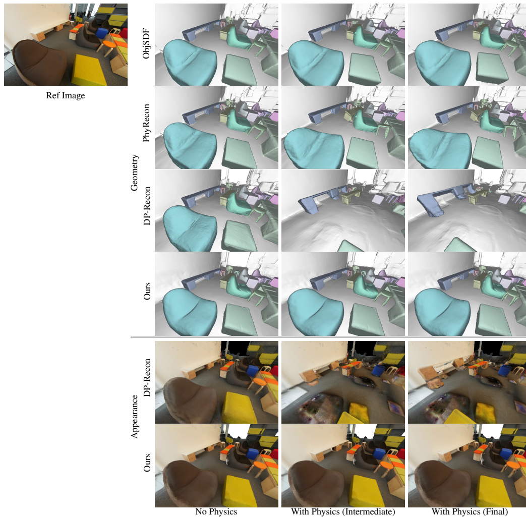
Figure 6: More Physical Simulation Results in Scannet++ Dataset Scene 2: We show the geometry and appearance of each object in the scene with physical simulation, from no physics state, intermediate state with physics, and final state with physics.
