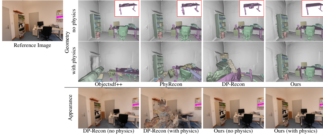
Figure 4: Qualitative Comparisons on Physical Simulation: We compare geometry layouts and appearance before and after physical simulation, with the table geometry reconstructions highlighted in inset figures. HoloScene’s complete, non-interpenetrating geometry remains stable in physics simulators, unlike baseline methods. Our Gaussian on mesh delivers high-quality, real-time rendering throughout the simulation process.
