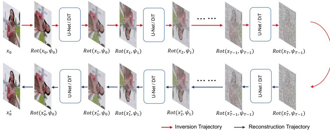
Figure 2: Detailed illustration of FreeInv. We employ rotation Rot(\cdot, \cdot) as the transformation f(\cdot) for example. During both the inversion and reconstruction phases, we rotate the latent representation with the same angle \psi_t at the t -th time-step, where \psi_t is randomly sampled.
