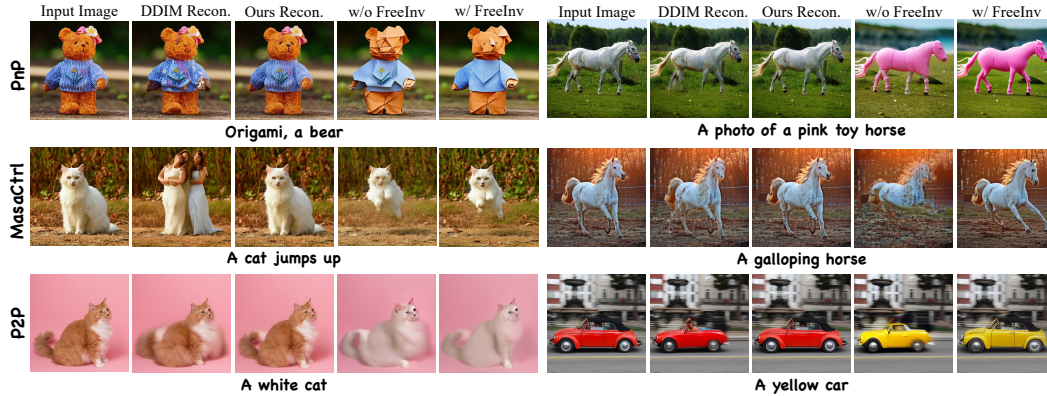
Figure 3: Qualitative comparison. We integrate FreeInv into PnP [42], MasaCtrl [4], and P2P [12], respectively. We compare the reconstruction and editing results w/ or w/o FreeInv.
