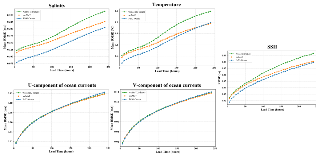
Figure 5: The ablation study of different methods on the HYCOM-RD. The five subplots respectively show salinity, temperature, ocean current UV components, and sea surface height. The x-axis represents the forecast lead time, and the y-axis represents the RMSE (lower is better). Note that for each variable, we average the RMSE over depth.
