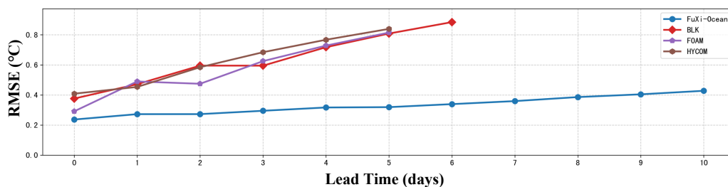
Figure 4: The SST comparison of different methods based on the IV-TT evaluation framework. The x-axis represents the forecast time, and the y-axis represents the RMSE (lower is better).
