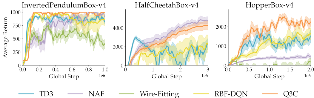
Figure 4: Restricted Environments. Q3C consistently outperforms TD3, RBF-DQN, and Wire-Fitting in restricted environments and largely outperforms NAF. Q3C converges at a higher reward with high stability while other algorithms are stuck at local optima.
