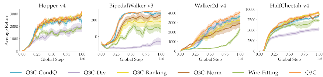
Figure 5: Ablations of Q3C. Every component of Q3C is validated for importance. Individual Q3C components complement each other and combined Q3C model visibly outperforms ablations.
