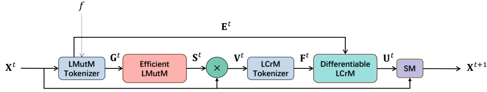
Figure 1: The overall framework of EPOM. The LMutM Tokenizer and LCrM Tokenizer are designed to generate input tokens for the Efficient LMutM and Differentiable LCrM, which are responsible for obtaining the mutant population \mathbf{V}^t and the candidate population \mathbf{U}^t , respectively. Finally, the SM produces the offspring population based on \mathbf{X}^t and \mathbf{U}^t .
