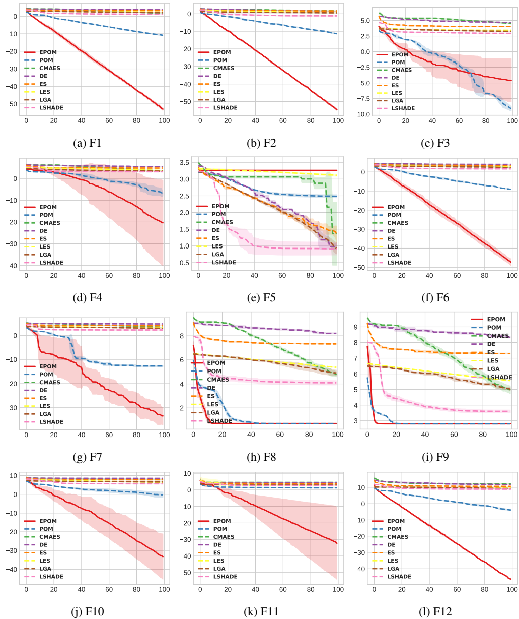
Figure 8: The log convergence curves of EPOM and other baselines on F1-F12. It shows the convergence curve of these algorithms on the functions in BBOB with d = 100 .
