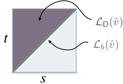
Figure 2: Self-distillation. Our plug-and-play approach pairs any distillation objective \mathcal{L}_{\text{D}} on the off-diagonal s \neq t of the square [0, 1]^2 with a flow matching objective \mathcal{L}_b on the diagonal s = t to obtain a direct training algorithm for the flow map.
