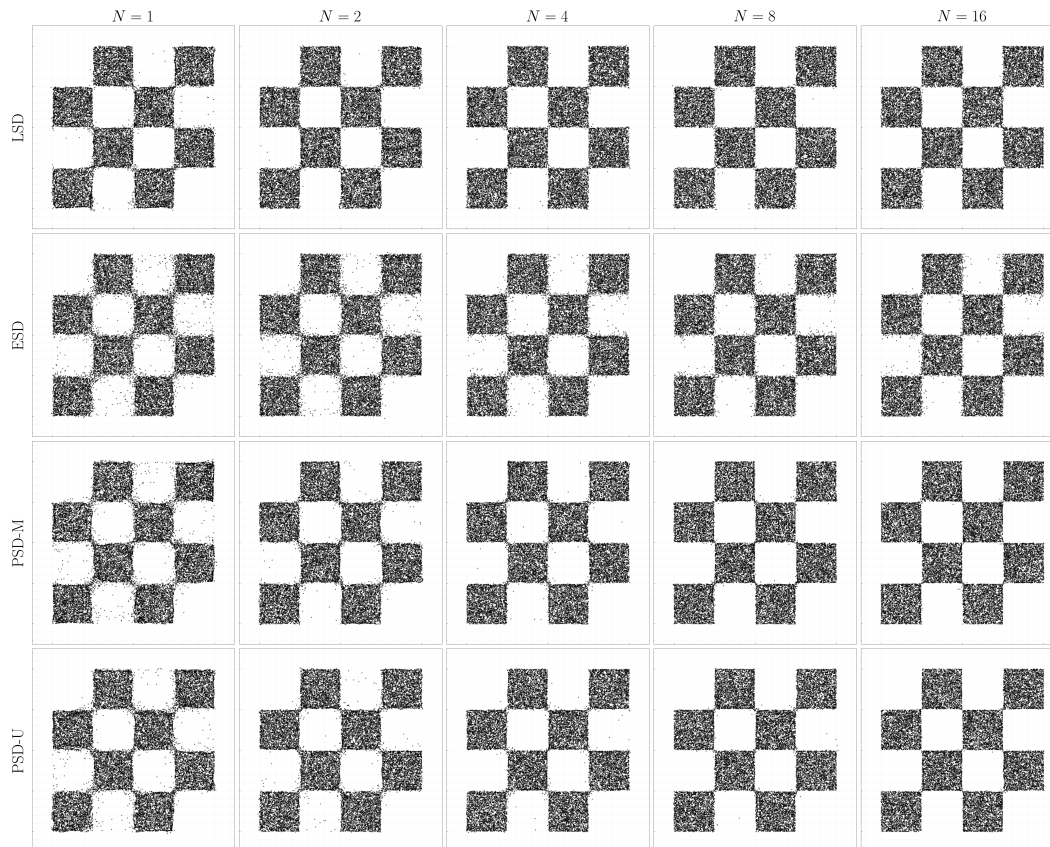
Figure 6: Checker: full qualitative results Full visualization of sample quality as a function of number of steps on the two-dimensional checker dataset.
