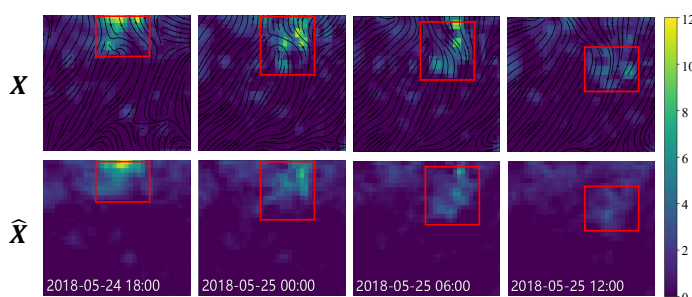
Figure 7: Visualization of PM_{2.5} concentrations as heatmaps. The first row shows reference distributions X overlaid with wind streamlines, and the second row shows model predictions \hat{X} . The spatial displacement of pollution illustrates how CTENet captures the dynamic advection of pollutants, consistent with atmospheric physical principles, and reflects the model's capacity to learn meaningful spatiotemporal interactions.
