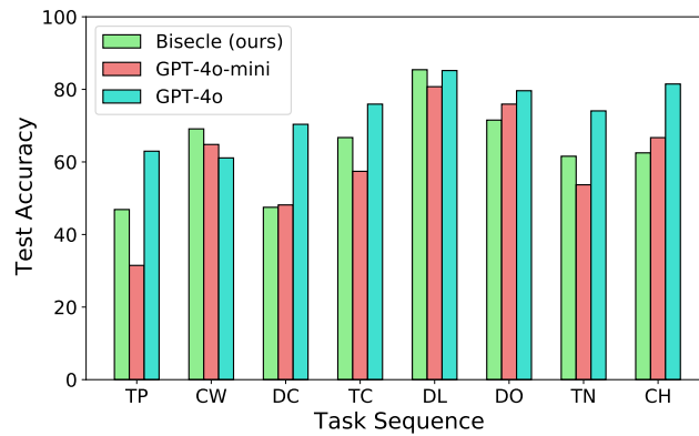
Figure 11: The performance of GPT-4o and GPT-4o-mini on the learning tasks of NExT-QA in our continual learning setting.
