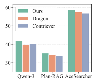
(b) HotpotQA
