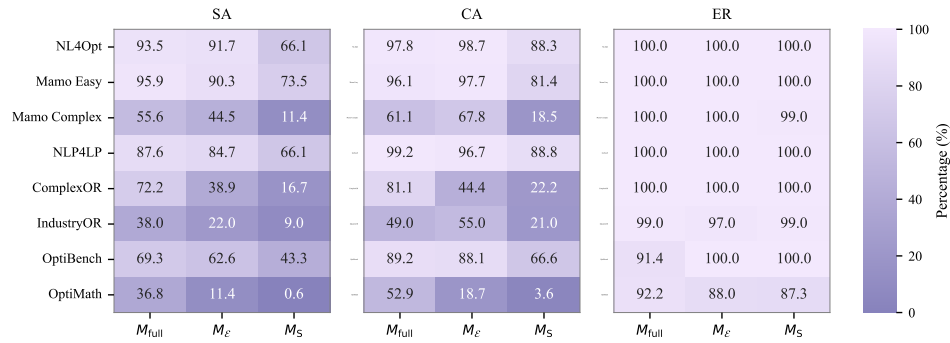
Figure 4: Heatmap of ablation study comparing M_{full} , M_E , and M_S across benchmark datasets. Deeper purple indicates poorer performance.
