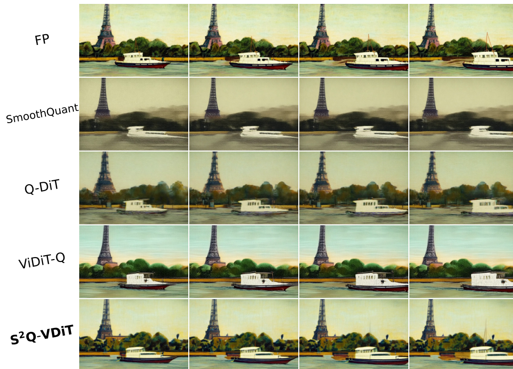
Figure 17: CogVideoX-2B results. Prompt: A boat sailing leisurely along the Seine River with the Eiffel Tower in background by Vincent van Gogh.
