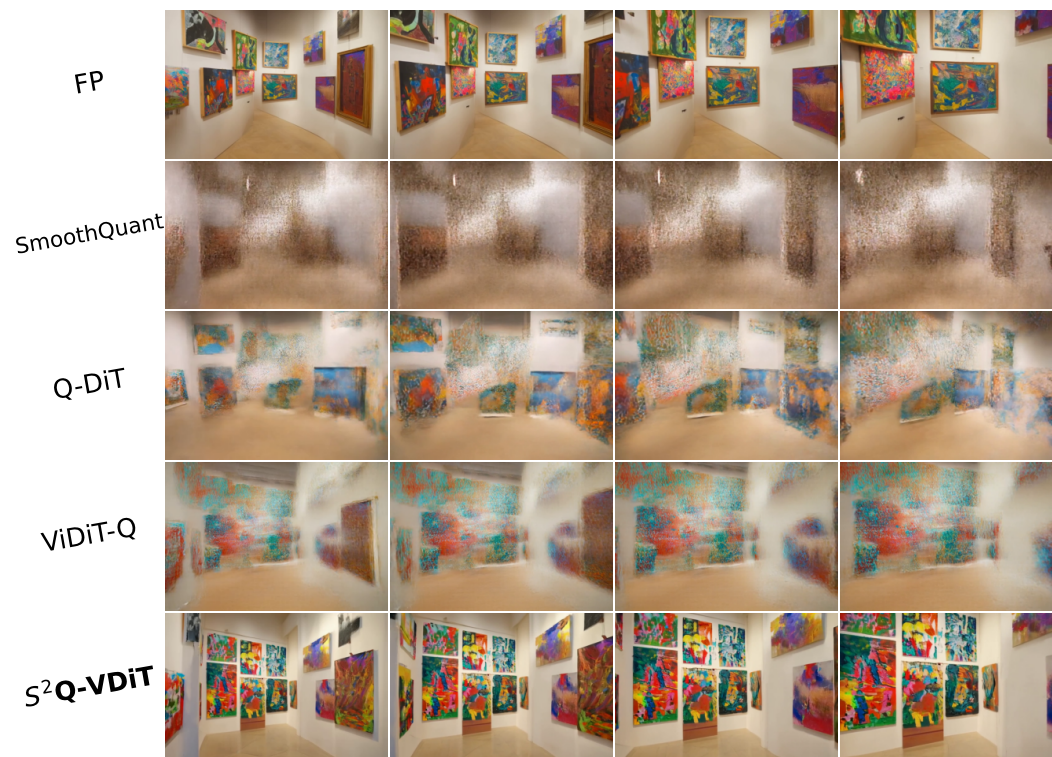
Figure 14: CogVideoX-5B results. Prompt: A modern art museum, with colorful paintings.
