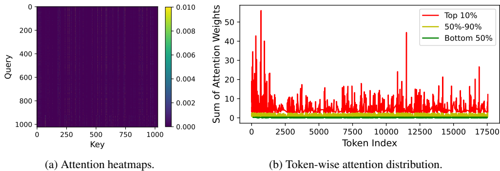
Figure 4: Visualization of sparse attention patterns in CogVideoX-2B block-10. In (4a), fewer columns have significantly higher weights. In (4b), only 10% of tokens have larger attention weights.
