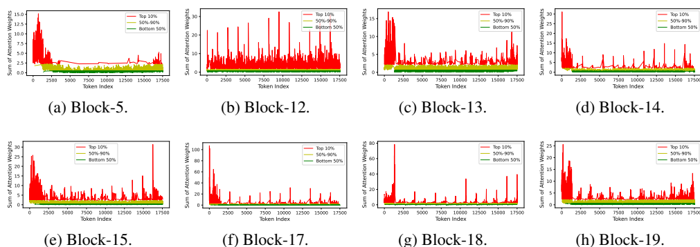
Figure 9: Visualization of token-wise attention distribution in CogVideoX-2B.
