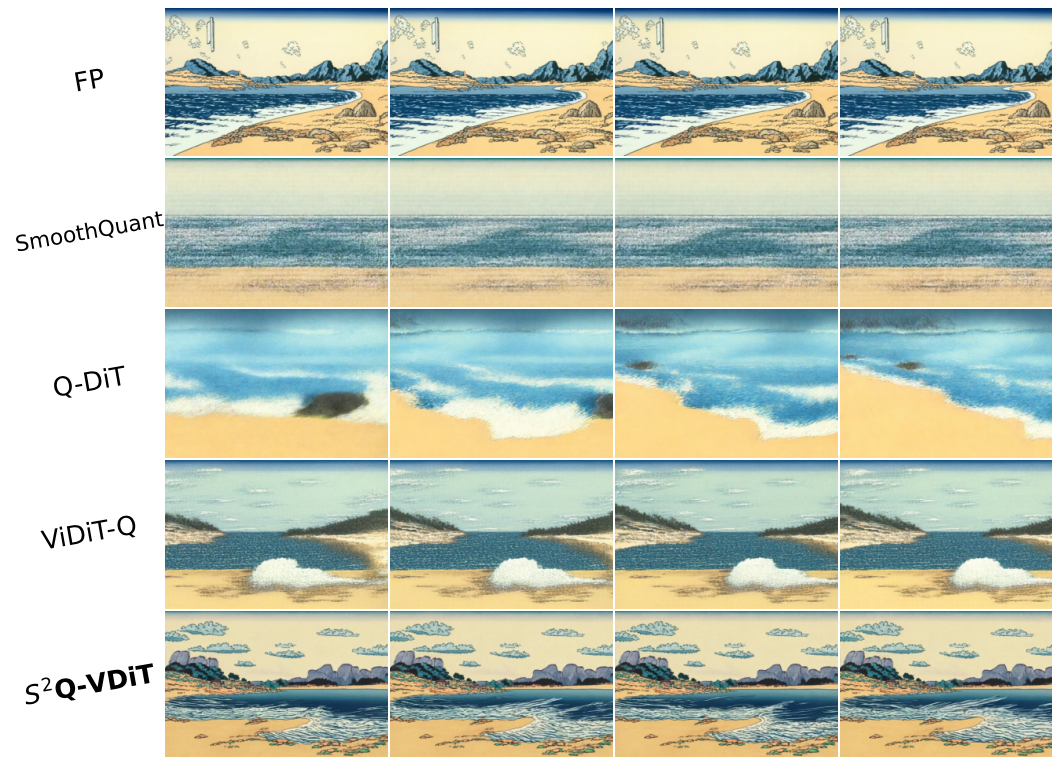
Figure 13: CogVideoX-5B results. Prompt: A beautiful coastal beach in spring, waves lapping on sand by Hokusai, in the style of Ukiyo.
