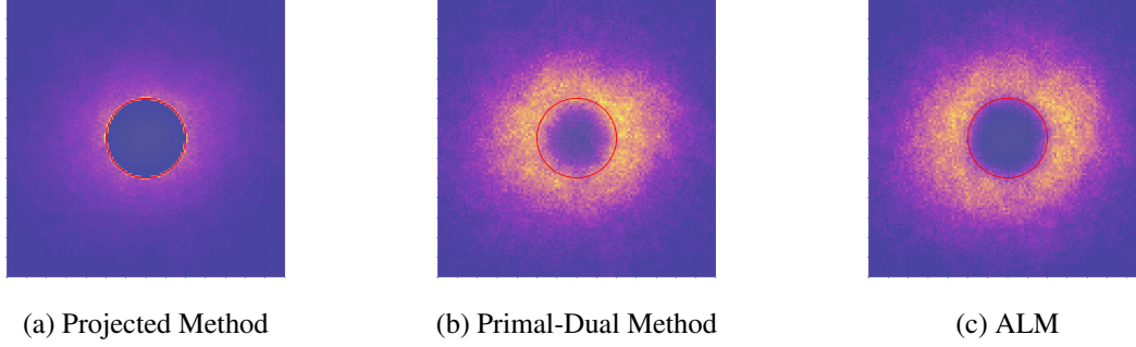
Figure 2: Constrained sampling trajectories through (a) projected, (b) primal-dual and (c) augmented Lagrangian Method. The goal is to use Langevin sampling methods to sample from a 2-dimensional Gaussian distribution with the constraint x^2 + y^2 \geq r^2 . Yellow regions show the high density of Langevin sampling trajectory distributions. Trajectories of the projected method mostly concentrate on the constraint boundary while the other two are more distributed.
