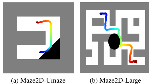
Figure 3: Trajectories generated by Constrained Diffuser in Maze2D Environment with Black obstacles. The blue part shows the start of the trajectories and the red part shows the target. We observe that the trajectories avoid the obstacles and reach the goal
