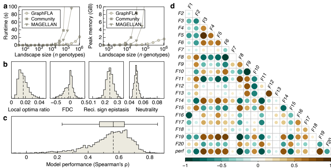
Figure 2: GraphFLA scales efficiently and captures influential landscape features for model performance. (a) Runtime (left) and peak memory usage (right) during fitness landscape construction for GraphFLA, MAGELLAN, and a community implementation [4], as a function of landscape size. Landscapes were generated using the NK model [70] by varying the number of loci N from 5 to 20 ( \rightarrow landscape sizes from 2^5 to 2^{20} ). Results shown are averages across 10 replicates. (b) Distribution of 3 representative landscape features across 155 combinatorially complete landscapes collected in GraphFLA. (c) Distribution of model performance, measured by Spearman's \rho , for Evo2 predictions across the same 155 landscapes. (d) Correlation matrix showing Spearman's \rho between 20 landscape features derived from GraphFLA and Evo2 performance across all 155 combinatorial landscapes.
