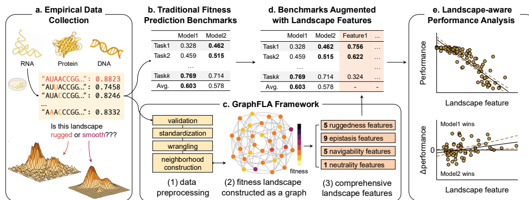
Figure 1: Overview of how GraphFLA contributes to the performance benchmarking of fitness prediction models. Existing biological fitness prediction benchmarks (b) are often curated from empirical fitness landscape datasets without interrogating landscape topography (a). GraphFLA constructs these landscapes and offers a comprehensive suite of features characterizing their topography (c). Such landscape features can then augment existing benchmarks (d) and thus assist performance interpretation (e, upper) and comparison (e, lower).
