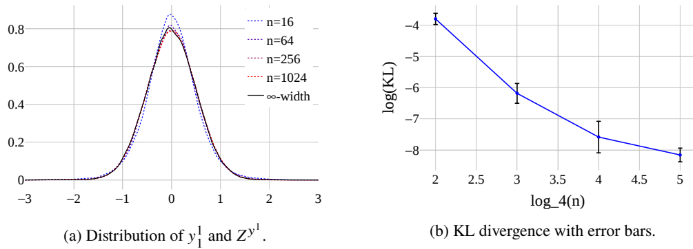
Figure 5: Comparison of the distribution of the attention output y_1^1 and its infinite-width limit Z^y with ReLU activation function. (a) Kernel density estimates of the empirical distribution (via Monte Carlo sampling) of y_1^1 for various widths n and head counts H (with n_H = n/H = 64 is fixed, dashed lines) alongside that of Z^y (solid lines). (b) Average of the log-KL divergence \log \text{KL}(\text{Dist}(y_1^1) \parallel \text{Dist}(Z^{y^1})) over 10 independent trials, plotted against \log_4(n) with error bars indicating one standard deviation.
