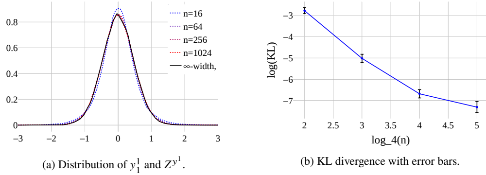
Figure 4: Comparison of the distribution of the attention output y_1^1 and its infinite-width limit Z^{y^1} when s = 8 . (a) Kernel density estimates of the empirical distribution (via Monte Carlo sampling) of y_1^1 for widths n \in \{16, 64, 256, 1024\} (dashed lines) alongside that of Z^{y^1} (solid line). (b) Average of the log-KL divergence \log \text{KL}(\text{Dist}(y_1^1) \parallel \text{Dist}(Z^{y^1})) over 10 independent trials, plotted against \log_4(n) with error bars indicating one standard deviation.
