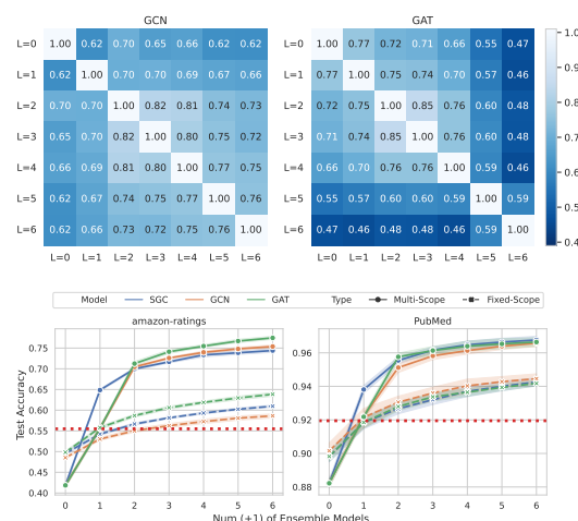
Figure 3: (Top) The overlapping ratio on Penn94. (Bottom) Test accuracy under Oracle ensemble. Multi-Scope represents the ensemble of GNNs with depths ranging from L = 0 (MLP) to n ( n \leq 6 ). Fixed-Scope represents the ensemble of GNNs with identical depth L = L_{\text{best}} . The horizontal red dotted line shows the SOTA GNN accuracy.
