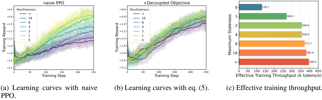
Figure 5: Ablation studies of the decoupled PPO objective and staleness control with a 1.5B model on math reasoning tasks. Both algorithmic choices are essential. With a moderate staleness value and the decoupled objective, training progress can be accelerated by over 2\times while maintaining final evaluation performance.
