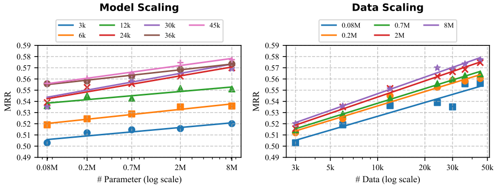
Figure 5: The illustration of the model and data scaling law of GFM-RAG.
