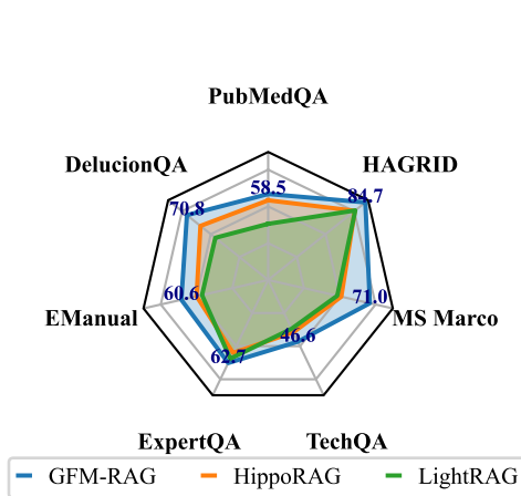
Figure 3: Model generalizability comparison.
