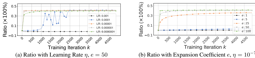
Figure 5: Ablation Studies of Improve Ratio to Learning Rate and Expansion Coefficient
