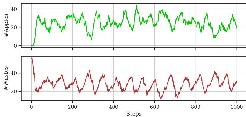
(d) Number of Apples and Wastes in the Environment
