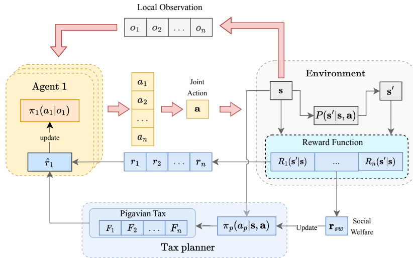
Figure 3: The Architecture of the LOPT . The centralized agent Tax planner allocate the Pigovian tax/allowance within a functional percentage formulation. Reward shaping is established based on the Pigovian tax/allowance to alleviate the social dilemmas.
