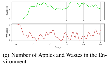
Figure 11: Number of Apples and Wastes in the Environment
