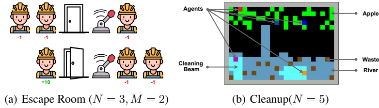
Figure 4: Environment Examples
