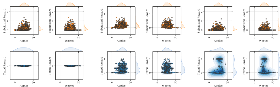
(a) Tax/Allowance Schemes with Environmental States for Cleaner Agents (b) Tax/Allowance Schemes with Environmental States for Harvester Agents (c) Tax/Allowance Schemes with Environmental States for Part-time Agents
