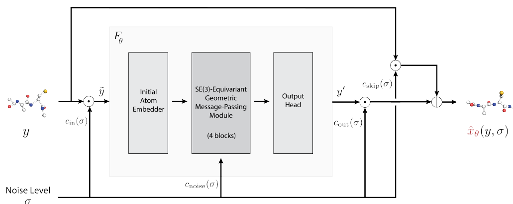
Figure 12: Overview of the denoiser network \hat{x}_\theta . The submodule F_\theta sees input atom coordinates \tilde{y} = c_{\text{in}}(\sigma)y and outputs predicted atom coordinates y' , which gets scaled and added to a noise-conditional skip connection to finally obtain \hat{x}_\theta(y, \sigma) .
