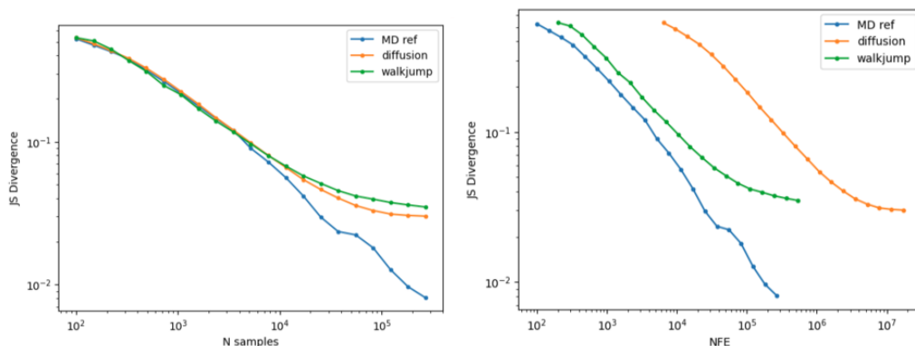
Figure 9: Comparison between diffusion, walk-jump and the ground truth MD in terms of JS divergence of backbone torsions to the full ground truth MD distributions, as a function of (left) number of samples and (right) number of function evaluations.
