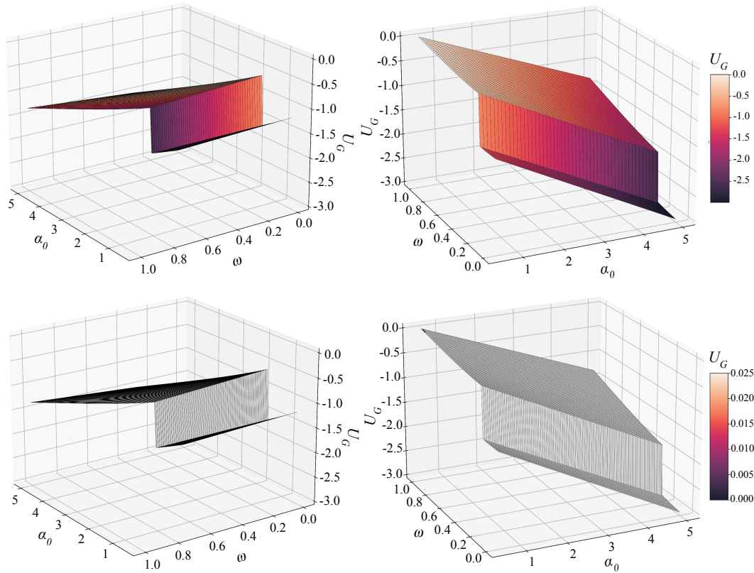
Figure 15: Generalist's strategy space for (\alpha_0, \omega) when |\epsilon - 1 - \delta| < c_\omega , with parameters \epsilon = 0.7, \delta = 0.1, c_\omega = 0.5, p = 1, \theta = 0.2 . (Top) G 's unconstrained strategy space for azimuth = 145 and azimuth = 245. (Bottom) G 's strategy space when abstaining for negative utility payoffs for azimuth = 145 and azimuth = 245.
