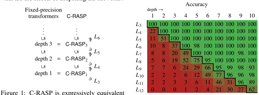
Figure 1: CRASP is expressively equivalent to fixed-precision transformers at each depth level. Then, because deeper C-RASP programs can solve more problems, deeper fixed-precision transformers can solve more problems as well.
