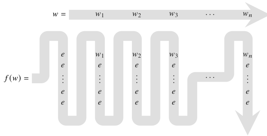
Figure 5: A set of x many formulas on a string w of length n can simulate a formula \phi on a string f(w) of length x(|w| + 1) .
