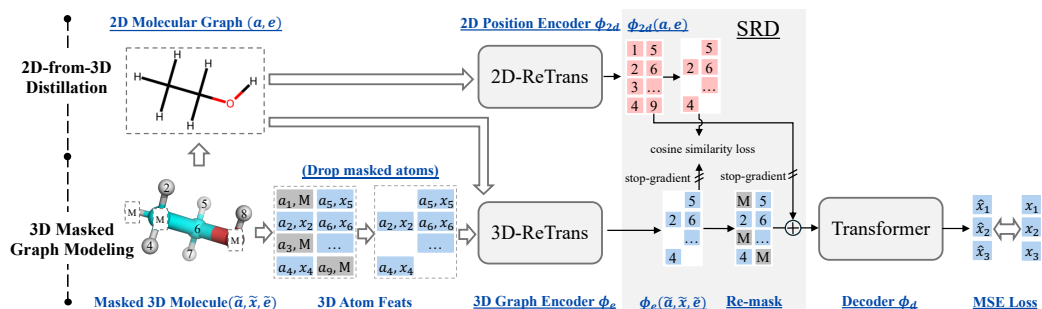
Figure 3: Overview of 3D-GSRD. It contains three key elements: (1) a 3D-ReTrans encoder; (2) the SRD that re-masks only 3D-relevant information from the encoder representations while preserving its 2D structure information via 2D-from-3D distillation; (3) a structure-independent decoder.
