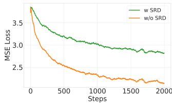
Figure 6: Probe encoder for masked atom coordinates when pretraining with/without SRD.
