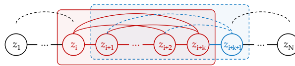
Figure 1: N instances with k -order dependency structure.
