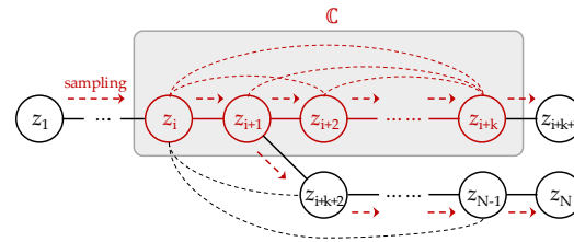
Figure 2: N instances with k -order dependency structure based on a tree-structured backbone.
