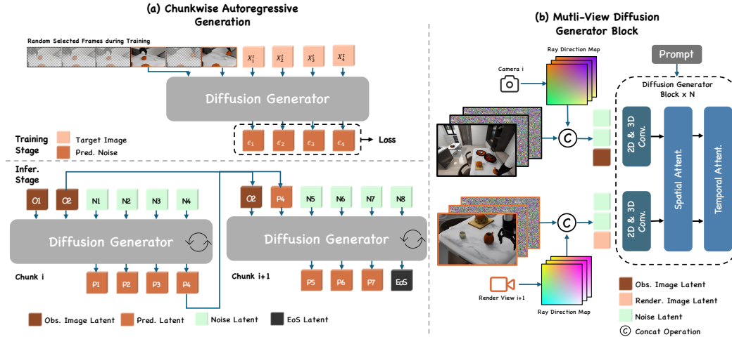
Figure 2: An overview of our chunk-wise autoregressive generation approach and multi-view diffusion generator block. (a) During training, random clean frames from consecutive sequences are combined with noisy frames to predict denoised latents. In inference, newly generated denoised frames become the next clean frames for subsequent steps, iterating until the EoS frame is detected. Only a single view of the autoregressive process is shown for clarity. (b) In the multi-view diffusion generator block, observational frames from Camera i or Rendered View i + 1 are encoded with a VAE. Ray direction maps are concatenated with video latents, followed by conv layers and attention mechanisms.
