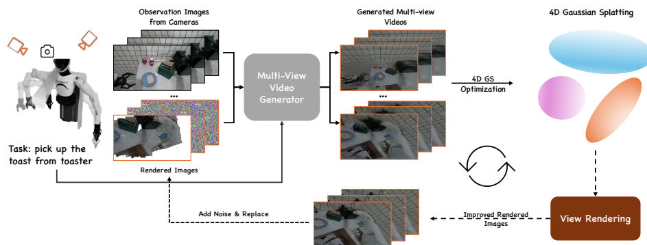
Figure 3: The pipeline for ENERVERSE as a data engine. Observation images from multiple cameras and rendered images are processed by the multi-view video generator to produce denoised videos. These videos, along with their camera poses, are used in 4DGS for 4D scene reconstruction. The reconstructed 3D content is rendered to generate high-precision images. These high-quality rendered images are iteratively refined and fed back into the pipeline.
