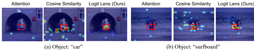
Figure 4: Object grounding results with LLaVA. Ground-truth bounding boxes are shown in red.
