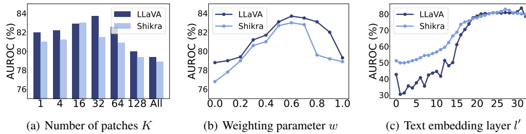
Figure 5: (a) Effect of the number of selected image patches K ; (b) effect of the weighting parameter w in Equation (5); and (c) effect of the text embedding layer index l' .
