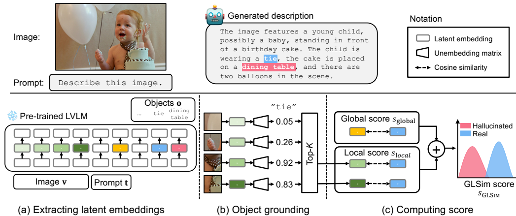
Figure 1: Overall framework. (a) We detect object-level hallucinations by leveraging latent embedding similarity. (b) For each object, the most relevant image regions are identified via unembedding from latent image representations. (c) The final GLSIM score is computed as a weighted combination of local (Section 4.2) and global (Section 4.3) signals, capturing both scene-level plausibility and spatial alignment, enhancing object hallucination detection accuracy.
