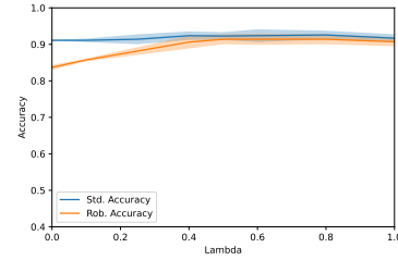
Figure 3: Accuracy as \lambda is increased from 0 to 1 for AAOpt on BPDA-EOT on CIFAR-10 ( \ell_\infty , \epsilon = 8/255 )
