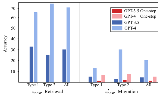
Figure 5: The semantic match accuracy of the target code snippets retrieval task and the target code snippets migration task across various LLMs. “One-step” indicates the direct utilization of an LLM to complete the migration task in a single step.
