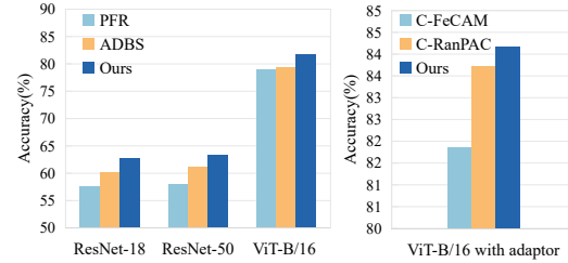
Figure 9: Accuracy after the last session on CUB200 with different backbones.
