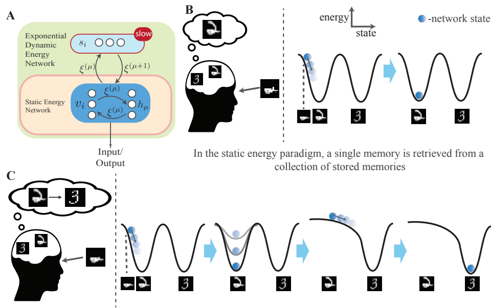
Figure 1: Schematic Model and Energy Landscape Behavior of Dynamic Energy Networks: A. The dynamic energy network, EDEN, has asymmetrically interacting slow neurons providing information about the next memory in the sequence to the two fast neural populations. B. Static energy-based networks are used as models of human associative memory where a single memory associated with a provided stimulus is recalled. EDEN, without the slow population, is a static energy network that retrieves a single memory from a collection of stored memories. The system's state ( v_i ), represented by the blue ball, descends the energy surface until a stable memory (energy minimum at state "2") is reached. After retrieval, the state of the system does not change and stays at "2". C. Dynamic energy networks enable associative sequence memory, where the associated memory along with its sequential neighbors are recalled. In EDEN, the energy surface changes in response to the state of the system, causing the minima of the energy surface to change over time (from "2" to "3"), resulting in transitions between memories.
