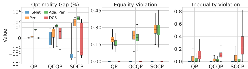
Figure B.3: Test results on 2000 instances of smooth nonconvex problems. FSNet consistently obtains near-zero constraint violations and small optimality gaps across the problem classes, whereas the baseline methods incur significant constraint violations.
