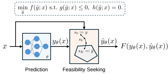
Figure 1: A schematic of FSNet, our framework for solving constrained optimization problems.
