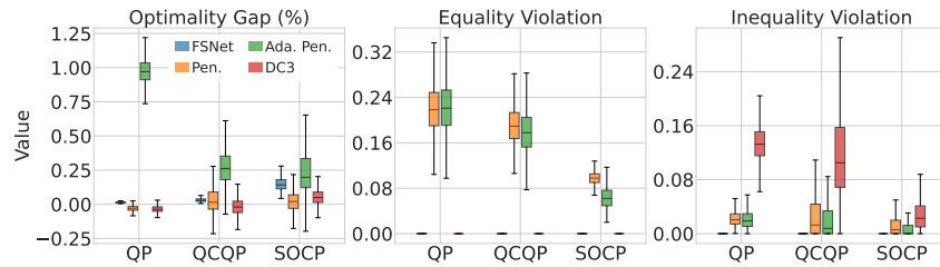
Figure 2: Test results on 2000 instances of convex problems with 100 decision variables. FSNet consistently obtains near-zero constraint violations and small optimality gaps across the problem classes, whereas the baseline methods incur significant constraint violations.
