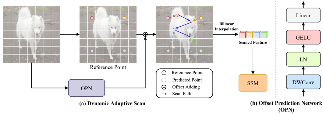
Figure 2: Illustration of the proposed Dynamic Adaptive Scan (DAS). For clarity, only four reference points are shown. Left: each initial reference point represents the original position of a patch, with its offsets learned by an Offset Prediction Network (OPN). Features of important regions are sampled based on the predicted 2D coordinates using bilinear interpolation. Right the detailed structure of the OPN is revealed. The query feature map is first transformed through depthwise convolution [22, 3] to integrate local information. Then, another linear layer, after layer normalization [1] and GELU [19] activation, converts the feature map into offset values.
