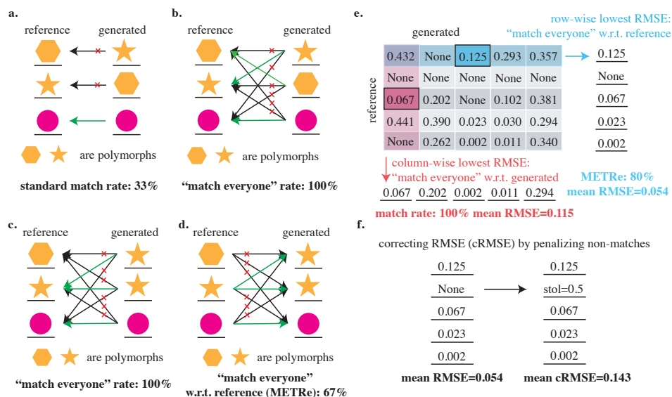
Figure 3: Demonstrating prior and new benchmarks. (a–d) A toy-case, in which the same colored shapes are considered polymorphs, shows different ways of computing match rate: (a) standard match rate, which penalizes polymorphs in the generated set being out of order; (b) "match everyone" metric, which fixes the fictitious penalty in (a); (c) a case of the "match everyone" metric in which a high match rate can be achieved without generating the diversity of polymorph structures; (d) our solution to the problems posed in (a) and (c), in which the number of matches from the "match everyone" metric is counted with respect to the reference set. (e) A demonstration of how "match everyone" differs when computed with respect to the generated vs. reference structures, showing that only the metric with respect to the reference structures (METRe) catches cases in which none of the generated structures match a given reference structure. (f) The implementation of corrected RMSE on a given matching metric.
