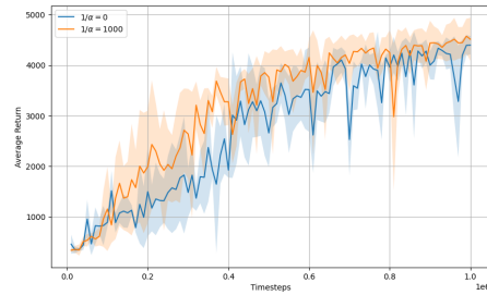
(b) Walker2d-v4: average return over 3 seeds
