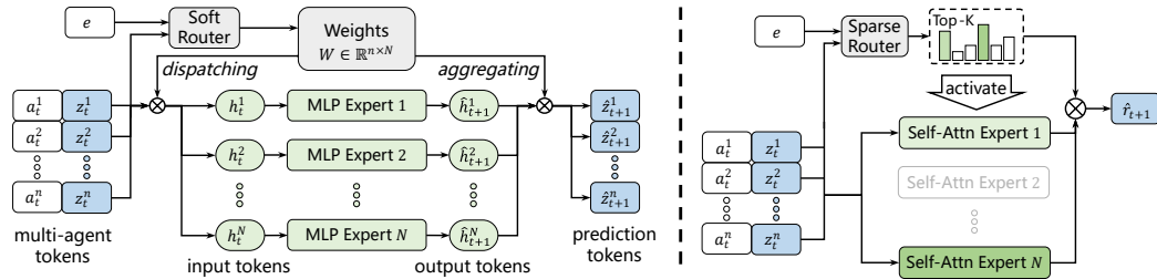
Figure 3: MoE in world model. The router generates a set of weights based on the task at hand, which is used for activating and allocating the experts. (Left) SoftMoE-based multi-agent dynamics model. (Right) SparseMoE-based reward predictor.
