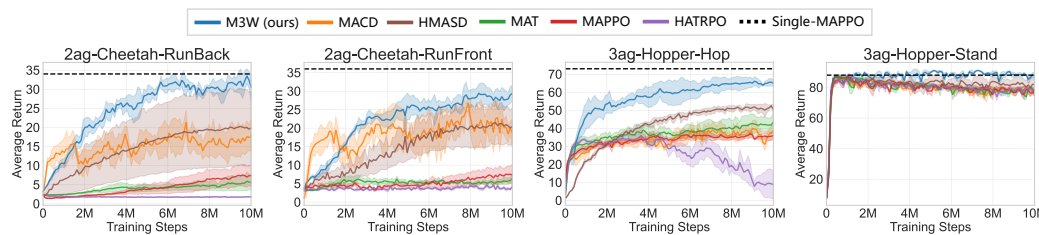
Figure 5: Performance comparisons for selected tasks in MA-Mujoco.
