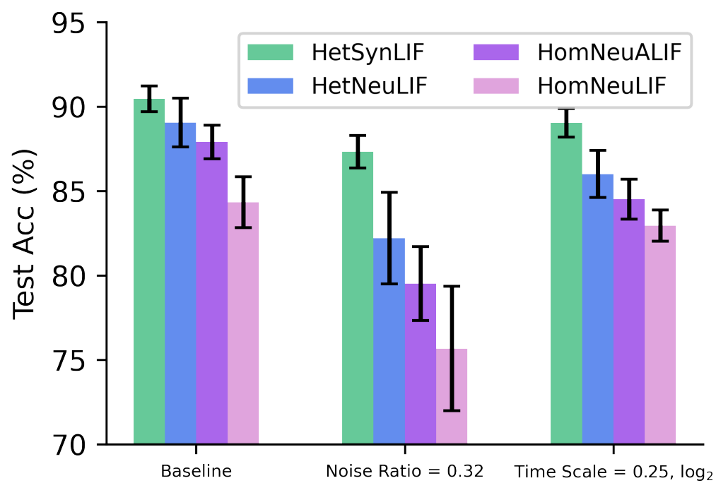
Figure A4: Bar plots show test accuracy of four RSNN variants on the SHD dataset under three conditions: baseline (left), deletion noise ratio 0.32 (middle, from Fig. 4C), and time warp scale 0.25 (log 2 , right, from Fig. 4F). Error bars represent standard deviation over 10 runs.
