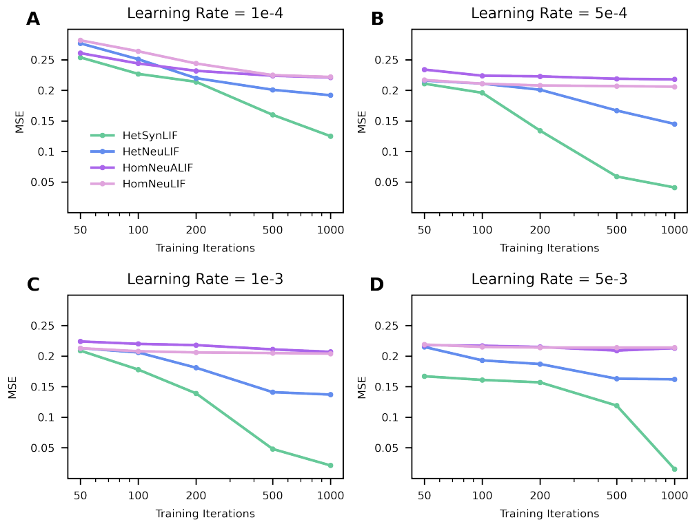
Figure A1: Convergence speed evaluation of four FSNN variants on the pattern generation task, trained with learning rates 1e-4 (A), 5e-4 (B), 1e-3 (C), 5e-3 (D). The curves show the mean squared error (MSE) over training iterations.
