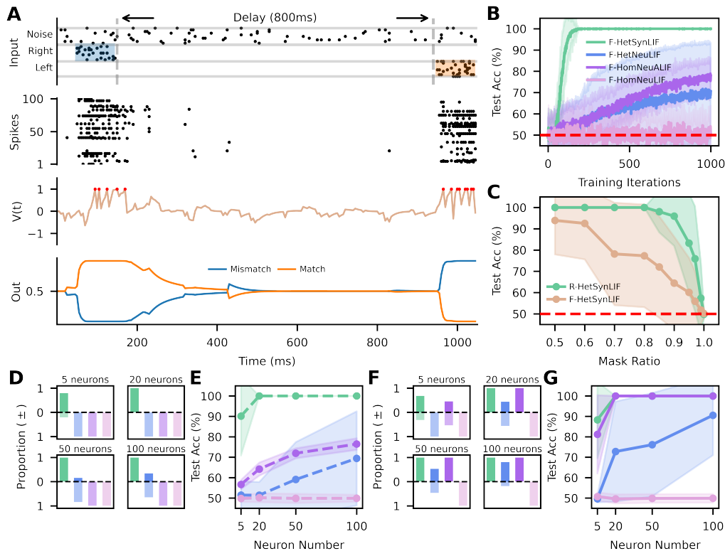
Figure 3: Delayed match-to-sample task. (A) Schematic diagram of a sample mismatch trial with two cues separated by an 800 ms delay (Top). Spiking activity of hidden layer neurons (Second). Membrane potential and spike activities (red dots) of a sample neuron (Third). Softmax outputs of neurons representing match and mismatch (Bottom). (B) Learning curves of four FSNN variants with 100 hidden neurons. (C) Task accuracy under different synaptic time constant masking ratios. (D) Success and failure rates across neuron numbers and FSNN variants. Each grid cell corresponds to a different hidden neuron count (5, 20, 50, 100), containing four centered bars for the four FSNN variants. Each bar is split vertically into a success segment (opaque, above) and a failure segment (transparent, below); trials with accuracy \geq 90\% are considered successful. D-G follow the same color scheme as B . (E) Overall task accuracy of four FSNN variants under varying neuron counts. (F-G) Same as D-E , but for RSNN variants. Data in B-G are averaged over 50 runs and reported as mean \pm s.d.
