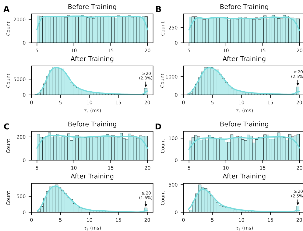
Figure A5: Distributions of synaptic time constants ( \tau_s ) across all connection types in the two-layer R-HetSynLIF. From (A) to (D): input to hidden layer 1, recurrent connections within hidden layer 1, hidden layer 1 to hidden layer 2, and recurrent connections within hidden layer 2. Each subplot shows the distribution of \tau_s before training (top) and after training (bottom).
