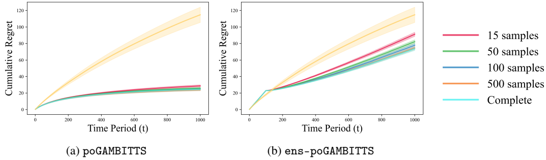
Figure 9: Cumulative Regret Under Varying Levels of Simulator Access
