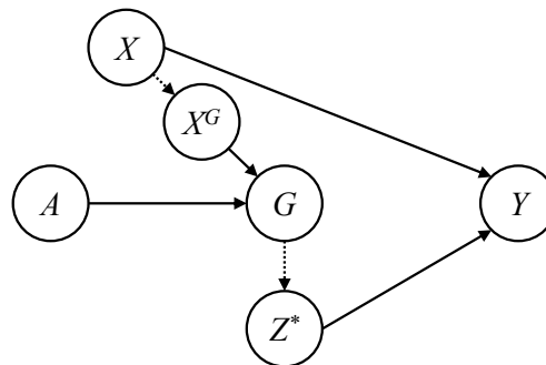
Figure 5: Generator-Mediated Bandit Causal Structure (Restricted Context in Query)
