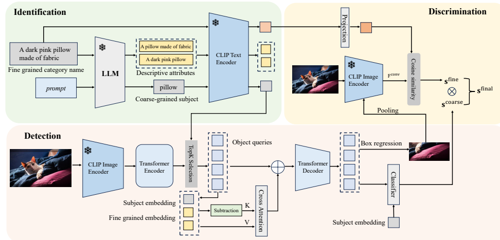
Figure 2: An overview of the proposed GUIDED framework. GUIDED adopts a three-stage pipeline, which consists of subject identification, coarse-grained object detection, and fine-grained attribute discrimination. In subject identification, GUIDED employs an LLM to extract the coarse-grained subject and its attribute embeddings. For detection, coarse-grained subject embeddings are adopted as queries to localize the candidate regions with coarse confidence. An attribute embedding fusion module selectively integrates attribute embeddings into queries. In the discrimination stage, GUIDED estimates the fine-grained score for each detected region with the full fine-grained class names using a refined CLIP with a projection head. The final score is obtained from the weighted multiplication of the detector's coarse confidence and the attribute similarity scores.
