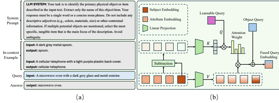
Figure 3: (a) Illustration of the prompt for subject identification. The prompt for extracting the associated attributes is shown in our supplementary document. (b) The architecture of the attribute-fused attention layer.
