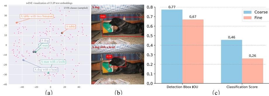
Figure 1: (a) The t-SNE visualization of CLIP text embeddings on LVIS classes and the fine-grained classes. The figure shows that some CLIP embeddings of fine-grained variants are positioned far apart. (b) The visualization of predictions of an OV detector with different class prompts (A dog vs A dog with a head). The detector focuses on the head instead of the dog, leading to incorrect localization. (c) The mean classification scores and the mean IoU of the prediction box with the ground truth box of OWL-ViT[24] under coarse-grained class queries and fine-grained class queries. The detector shows better performance on both classification and localization with coarse-grained queries than with fine-grained queries.
