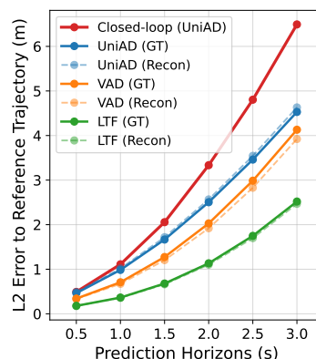
Figure 2: Comparison of average L2 error in the motion prediction under different prediction horizons.
