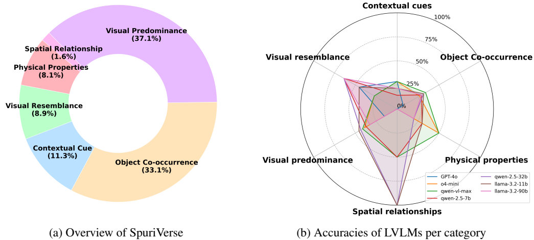
Figure 3: Categories of spurious correlations. Visual predominance and Object co-occurrence make up 37.1%, 33.1% of SpuriVerse, respectively. Only 2 spurious correlations fall under Spatial relationships. LVLMs tend to do better on Visual resemblance and Spatial relationships, achieving more than 50% accuracy, and achieve less than 50% accuracy on all other categories.
