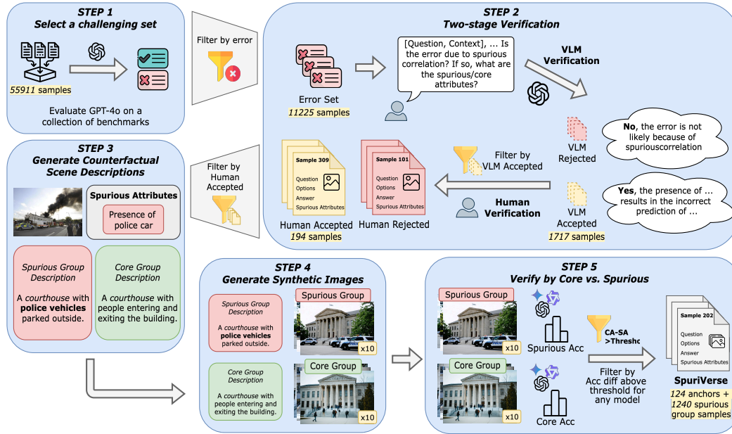
Figure 2: Curating SpuriVerse consists of 5 steps: (1) Derive errors from GPT-4o on a set of multi-modal multiple choice question benchmarks. (2) Two-stage Verification: (a) Prompt GPT-4o to identify errors attributable to spurious correlation and report the candidate spurious feature, and (b) Human verify the attribution and refine the spurious features if necessary. (3) Prompt GPT-4o to generate two scene descriptions based on the correct answer, one with and one without the spurious feature. (4) Generate 10 synthetic images for each description in pairs using Stable Diffusion, forming spurious and core groups for each sample. (5) Evaluate multiple LVLMs on both groups, and select those samples for which the accuracy difference is at least 30% for any model.
