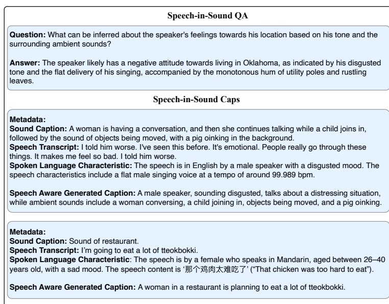
Figure 6: Examples of Speech-in-Sound Caps and QA , together with the metadata used for generating them.
