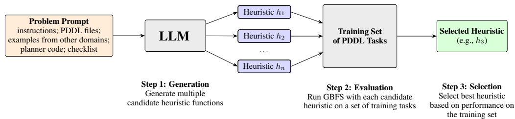
Figure 1: Our pipeline for generating domain-dependent heuristics with LLMs: we prompt the LLM n times to generate n candidate heuristics, evaluate each of these heuristics on a set of training tasks and choose the strongest one.
