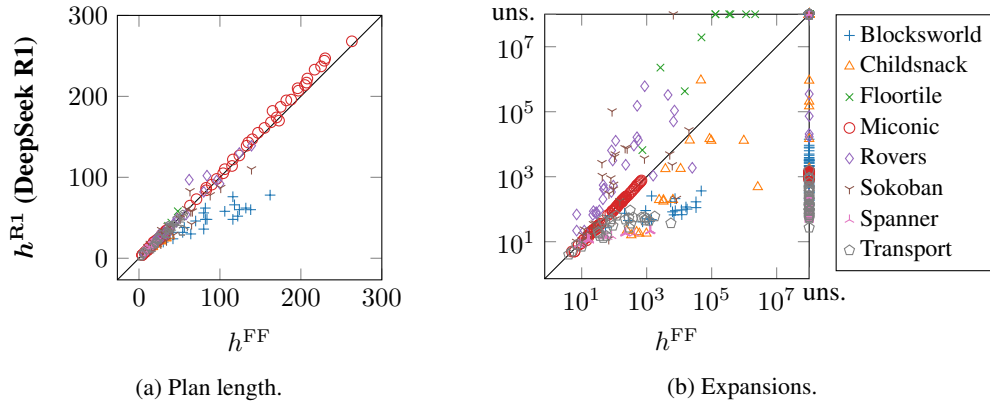
Figure 2: Comparison of plan length and expansions for h^{\text{FF}} and the heuristics generated by DeepSeek R1. We only show plan lengths up to 300 (only plans in Miconic exceed this limit).
