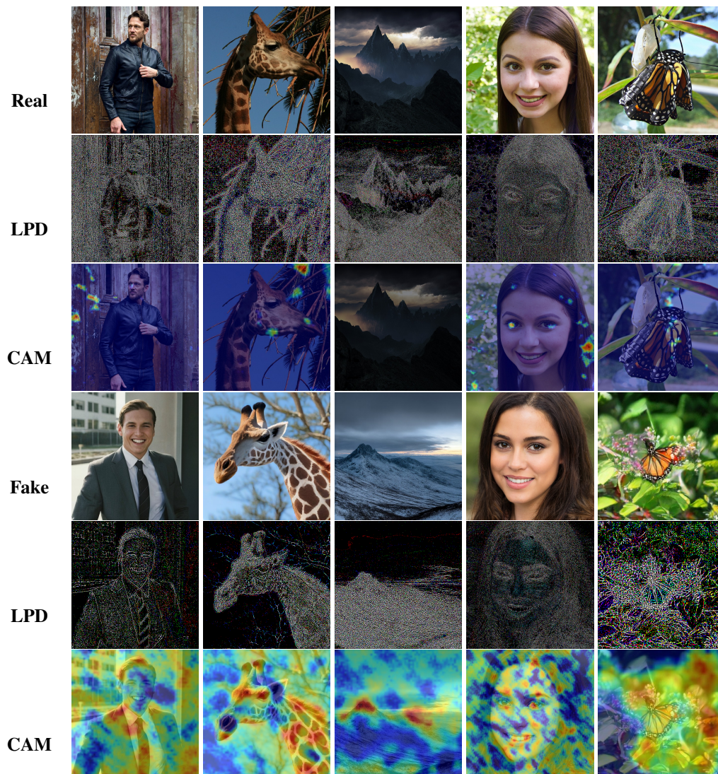
Figure 5: LPD and Grad-CAM visualizations of real and fake images.
