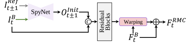
Figure 5: Overview of the reference-guided motion compensation (RMC) module.
