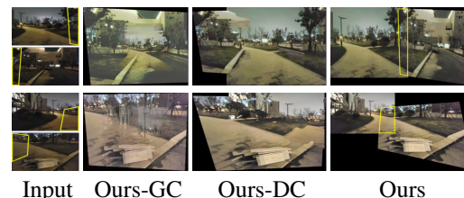
Figure 8: Visualization results for the ablation study on the RPHE.
