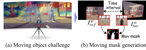
Figure 3: The generation process of the motion mask during image capturing.
