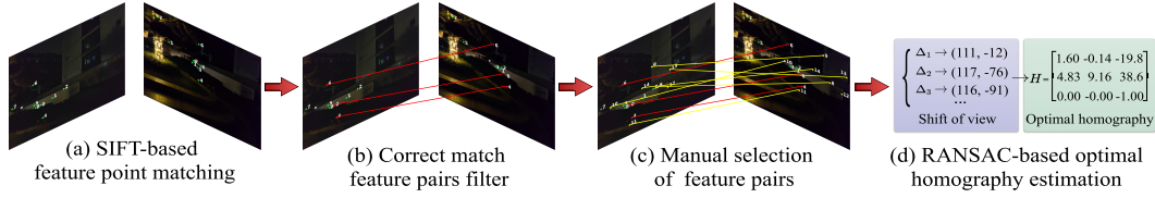
Figure 4: Reference generation process of the newly proposed ASIS dataset.
