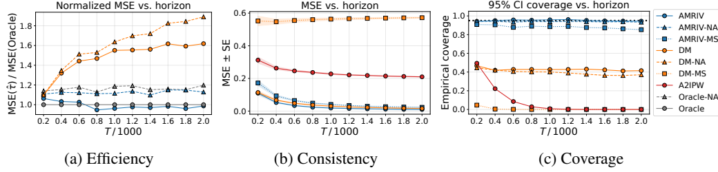
Figure 3: Performance of different estimators across increasing sample size T . (a) Efficiency: Normalized MSE versus an oracle benchmark. (b) Consistency: \text{MSE} \pm \text{standard error} . (c) Coverage: Empirical coverage of 95% confidence intervals.
