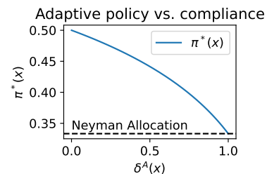
Figure 2: Optimal policy \pi^*(X) as a function of compliance \delta^A(X) .
