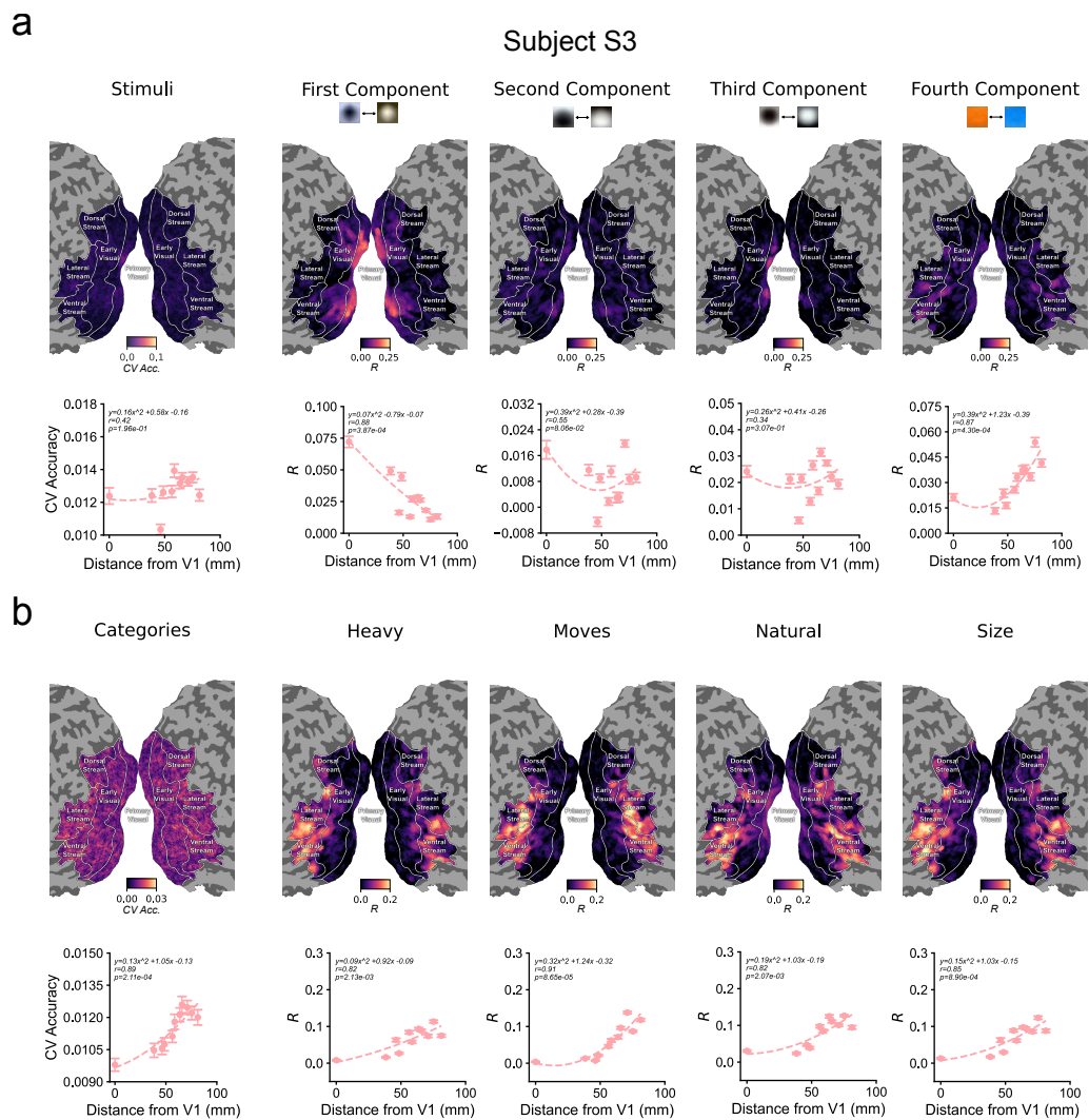
Figure A10: Low-level (a) and high-level (b) feature decoding in THINGS Subject 3.
