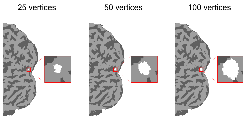
Figure A14: Representation of the size of the searchlight on the cortical flatmap for Subject 1 from the THINGS fMRI dataset: 25, 50, and 100 vertices.
