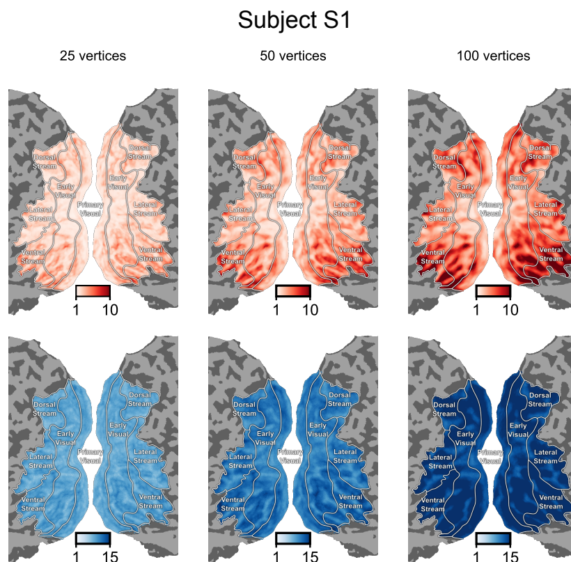
Figure A15: Lower dimensionality with smaller neighborhood sizes. For the neighborhood sizes shown in Fig. A14, we again compute the dimensionality across the whole visual cortex, and observe similar patterns as reported in the main text.
