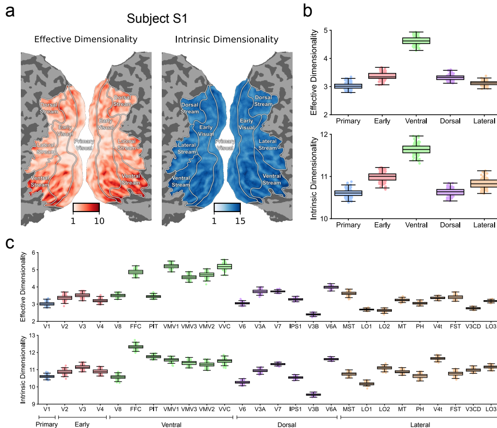
Figure 1: Dimensionality varies across cortex. a) Effective (ED) and intrinsic (ID) dimensionality across the visual cortex for subject S1 from THINGS fMRI dataset. Dimensionality was computed using a searchlight approach with 50 vertices (see Methods). Dimensionality averaged across larger brain regions ( b ) and smaller sub-regions ( c ). The boxes show the quartiles of dimensionality across searchlight discs in an area.
