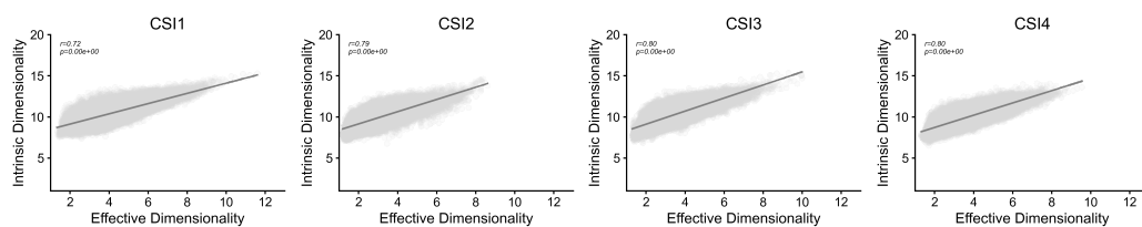
Figure A7: Correlation between effective and intrinsic dimensionality of vertices for BOLD5000 subjects.
