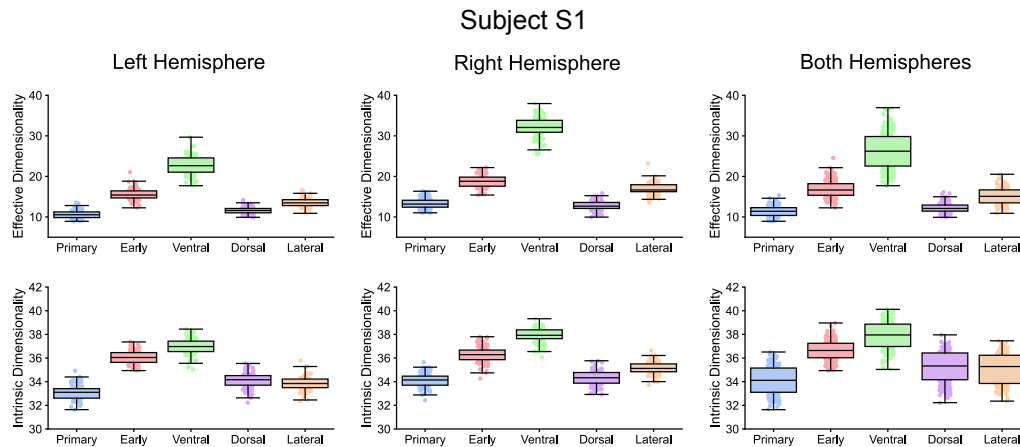
Figure A17: Calculation of dimensionality sampling random vertices of the different areas instead of using neighbors of vertices. Top: effective dimensionality, bottom: intrinsic dimensionality.
