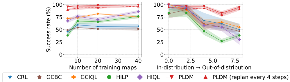
Figure 11: Evaluating PLDM’s performance under fixed inference time compute budget on diverse maze. Similarly to two-rooms, we only see a minor degradation in performance
